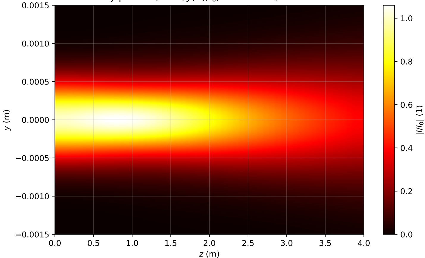
Intensity profile I(x=0, y, z)/I_0 , P_{in}=0.5P_{cr} , artificial time
